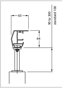
Standard Fix
