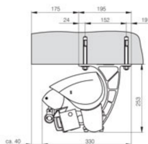
Ceiling mounting (Dimensions in mm)
